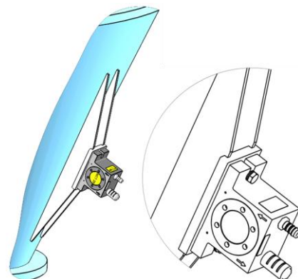
Mounting on weld-on console
